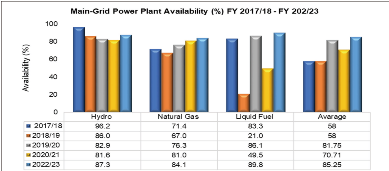
Figure 7: Main Grid Power Plant Availability (%) from 2017/19 to 2022/23
