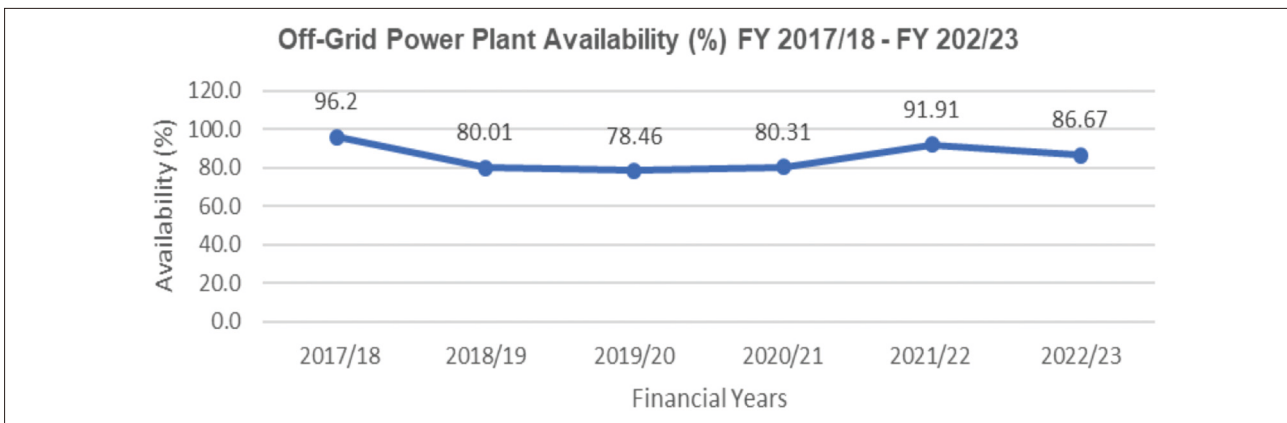
Figure 8: Off-grid power plant availability (%) FY 2017/18 - FY 2022/23
